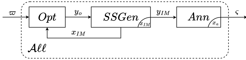
Figure 7.12: Block diagram of a dynamic allocator achieving full output invisibility as requested by Theorem 7.7: the optimizer, steady-state generator, and annihilator subsystems are represented by the blocks Opt , SSGen , and Ann , respectively.
