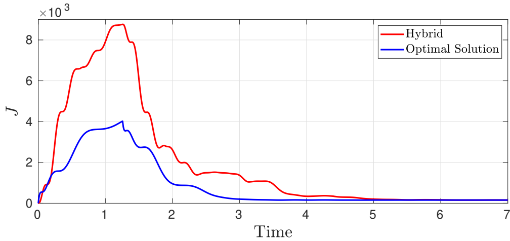
Figure 7.4: Cost in the presence of input allocation by means of a hybrid allocator (red), and of the periodic extension of the optimal solution to Theorem 7.10 (blue).
