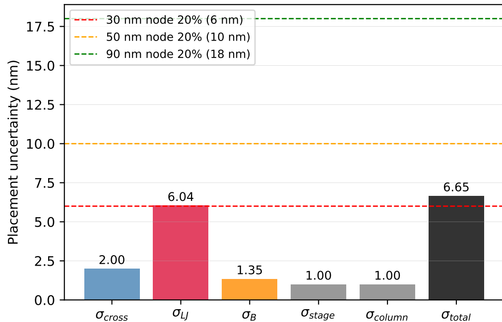
(b) v4 placement budget breakdown ( I_b = 2 nA quadrature)
