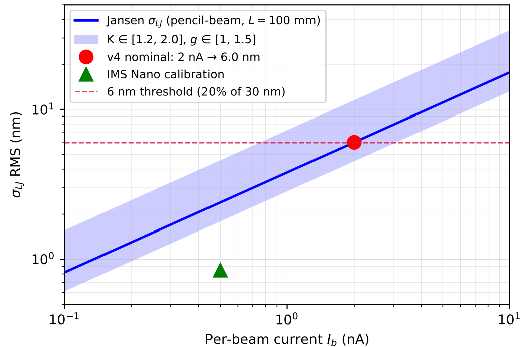
(a) Loeffler-Jansen vs current at v4 geometry ( V_0 = 50 kV, L = 100 mm)
