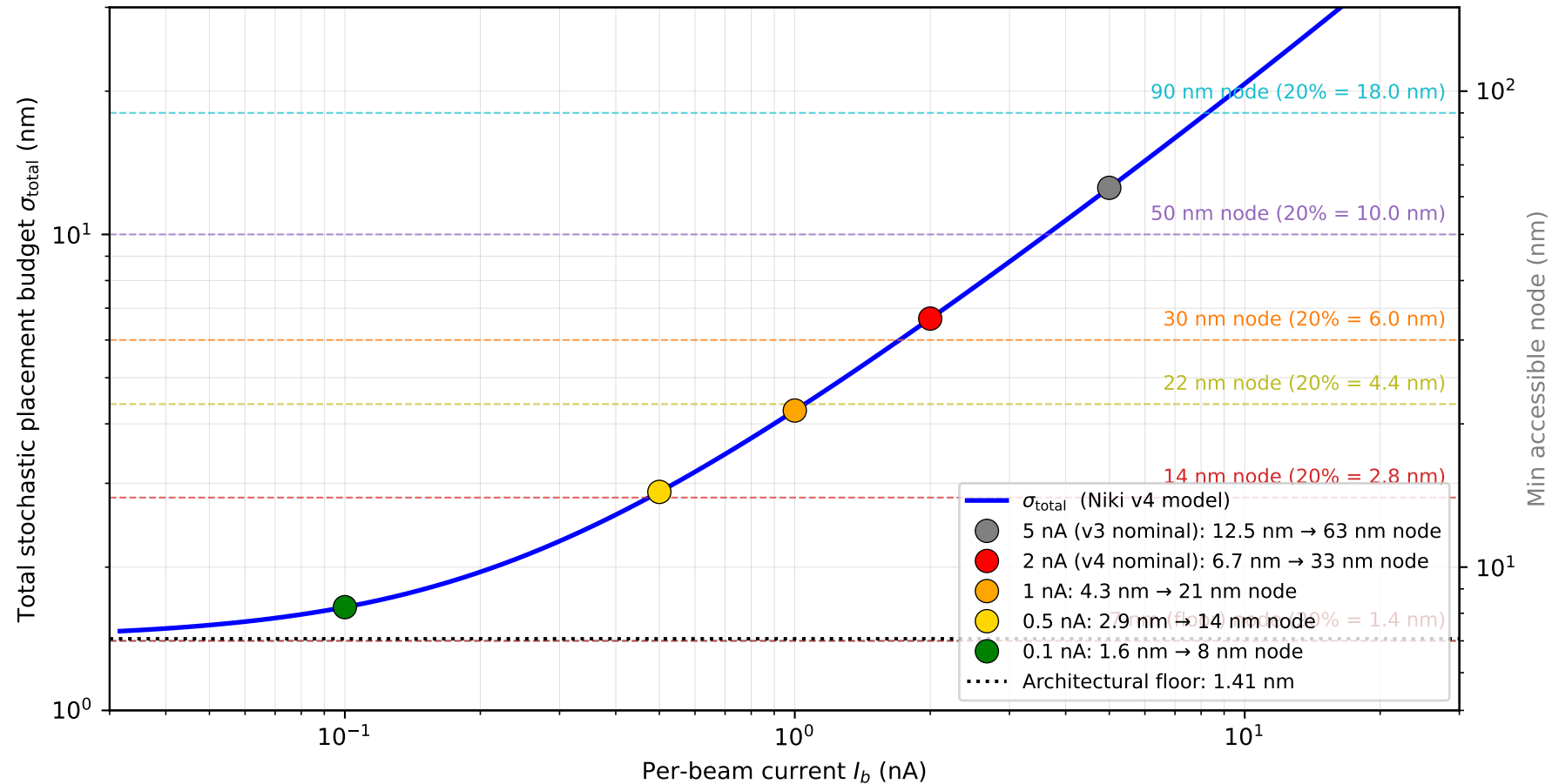
v4 architecture — node accessibility vs per-beam current ( V_0 = 50 kV, L = 100 mm, N = 10^6 , P = 20 \mu\text{m} ; \sigma floor = stage + column optics only)
