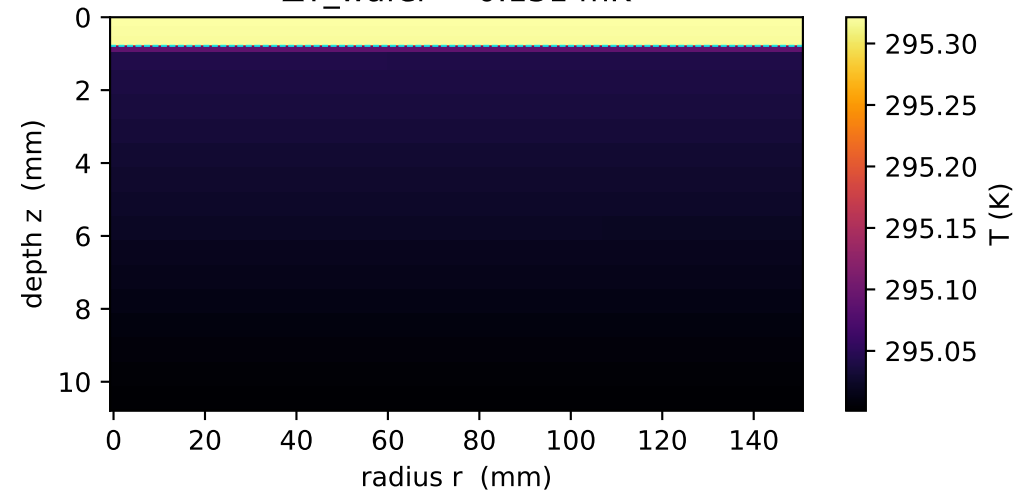
(b) T(r,z) -- SCANNED uniform 920 W/m 2 (spec mode), TEC ON \Delta T_{\text{wafer}} = 0.131 mK
