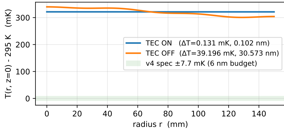
(c) SCANNED case -- wafer-top profile (the spec)
