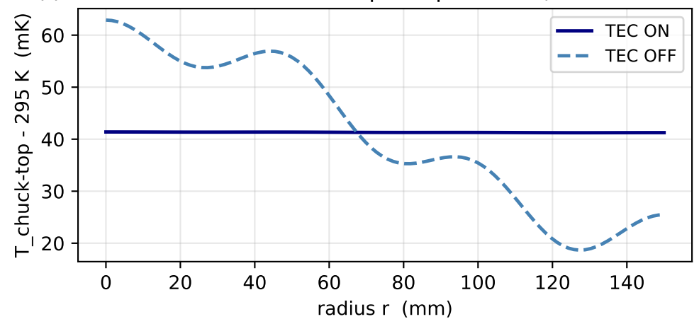
(f) SCANNED case -- chuck-top temperature (Dirichlet-driven)
