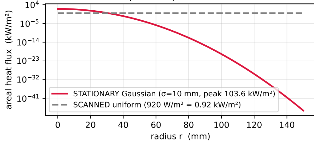
(e) Beam-deposition profiles, 65 W total each
