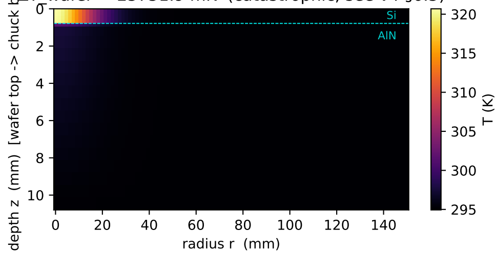
(a) T(r,z) -- STATIONARY column (Gaussian \sigma=10 mm), TEC ON \Delta T_{\text{wafer}} = 25751.9 mK (catastrophic, see v4 §6.5)
