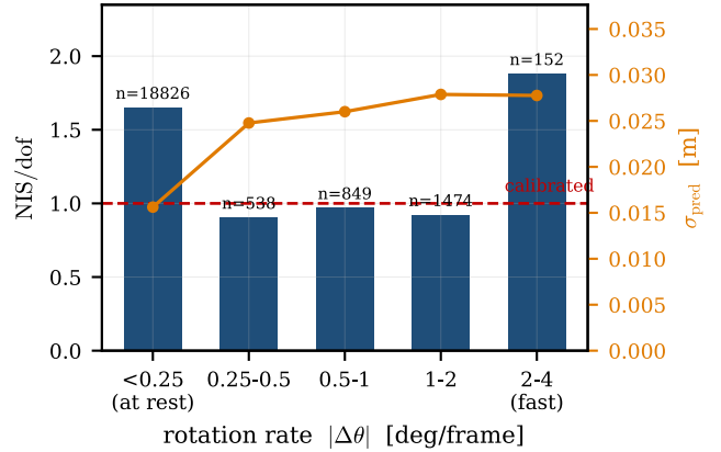
Fig. 4. The channel is calibrated only while the robot moves. NIS per rotation band over a 200 m tour, with the pose-induced corner uncertainty \sigma_{\text{pred}} overlaid. Three independent bands of genuine motion sit at 0.90 to 0.97. At rest \sigma_{\text{pred}} collapses while the innovation grows, and under fast rotation the innovation grows again—two distinct mechanisms bracketing a correctly calibrated middle.
