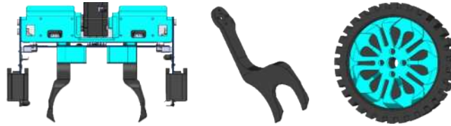
Figure 5. 3D-printed rescue and drive parts: (a) arm, (b) gripper, (c) wheel with EPDM-foam tire.
