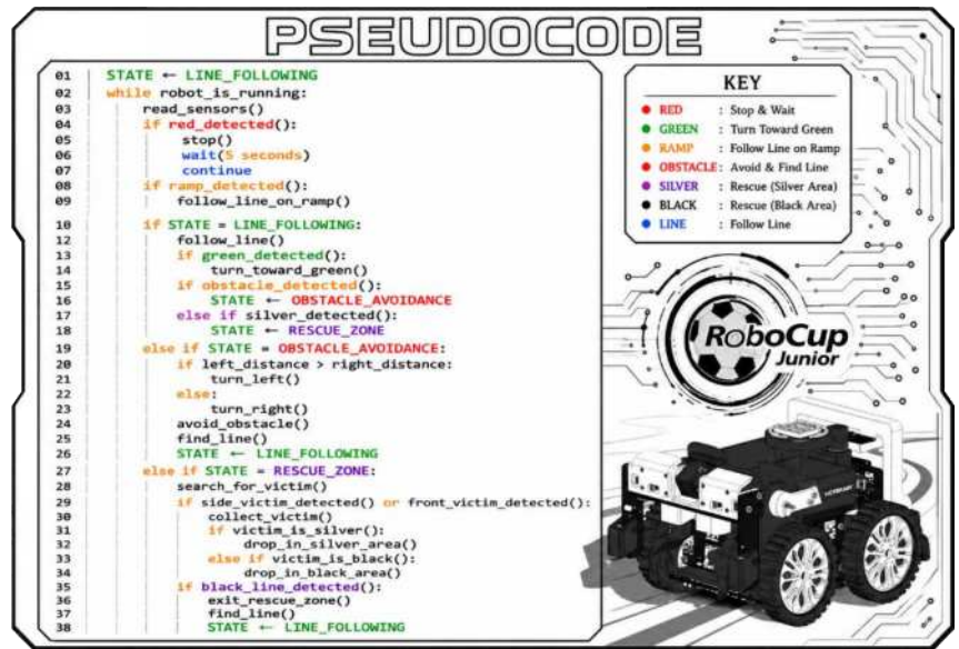
Figure 16. Robot full control PSEUDOCODE.
