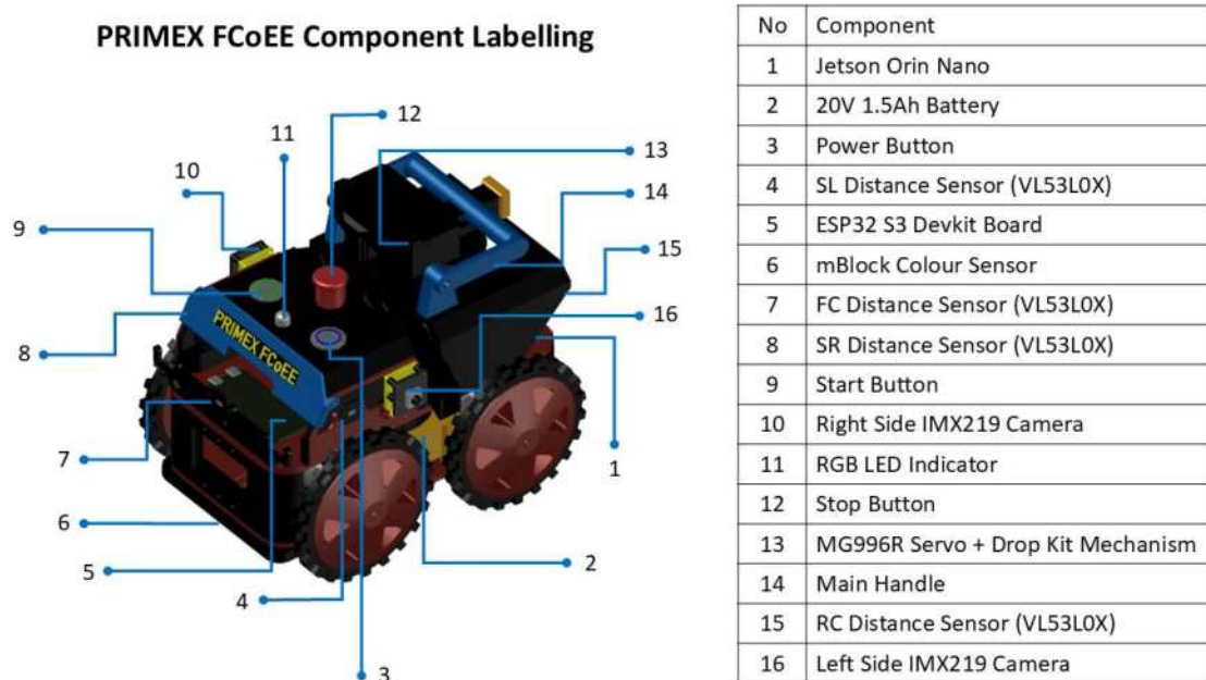
Figure 3 : PRIMEX FCoEE Full Robot Configuration with Component Labelling
