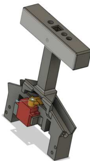
Figure 3: CAD view of the directional rescue-kit mechanism with servo-driven release geometry and vertical storage tower.
