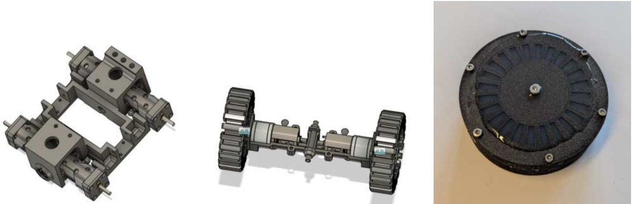
Figure 2: Drive-train details. Left: motor and shaft mounting without the upper structure. Center: axle module with wheels and central shaft linkage. Right: finished custom wheel with cast silicone tire mounted on the printed rim.
