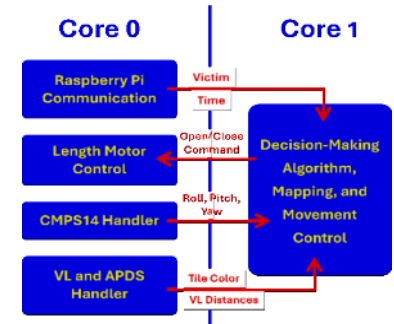
Task distribution and Data flow across ESP32 cores using FreeRTOS.
