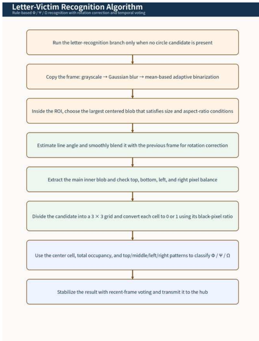
Figure S4. Rotation-corrected, 3 \times 3 pattern-based recognition of Phi, Psi, and Omega.
