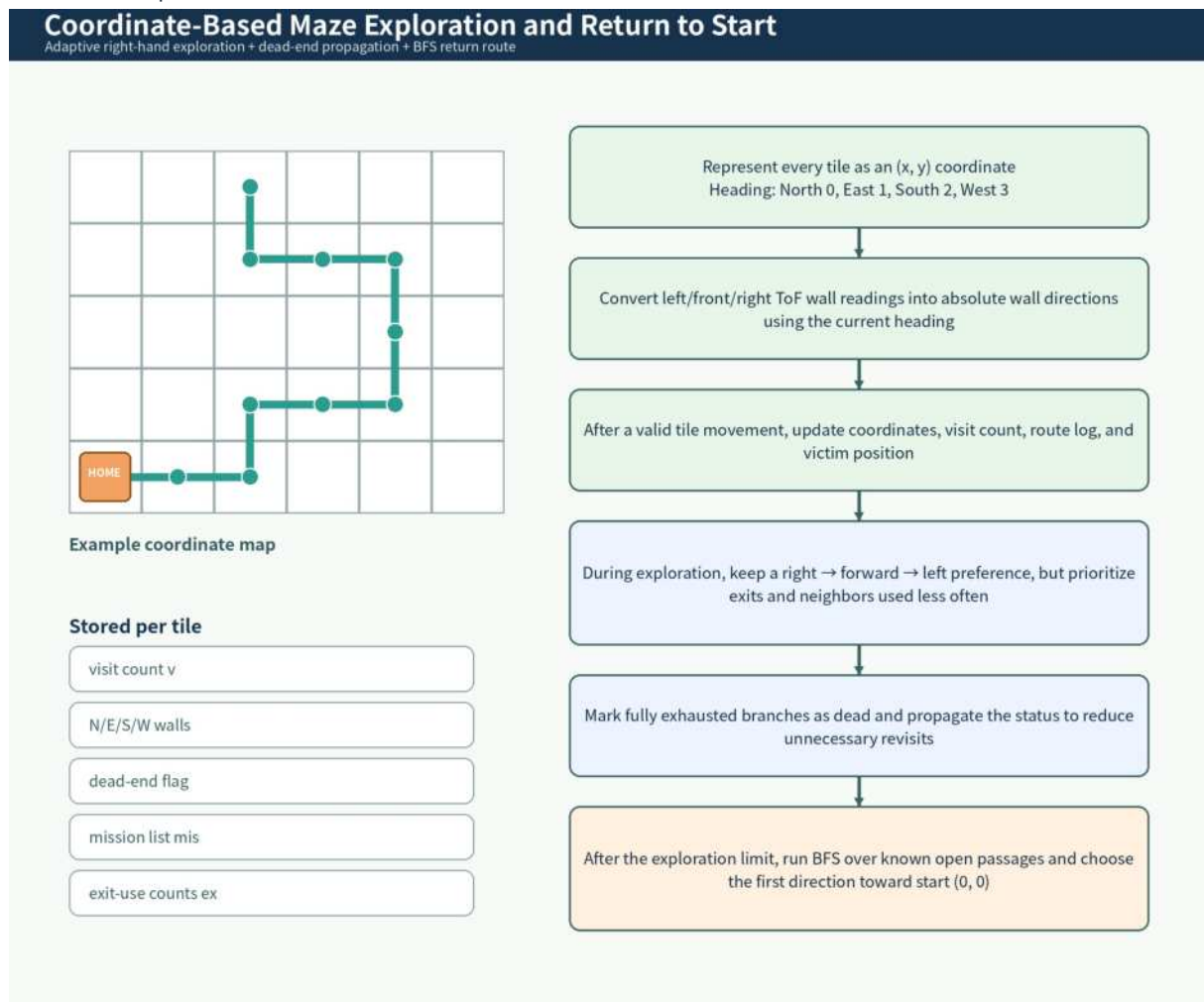
Figure S2. Coordinate-map generation, adaptive exploration, dead-end propagation, and BFS return.
