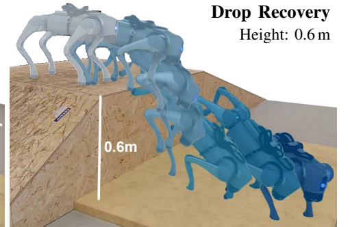
Fig. 8: Robust locomotion during slope traversal and drop recovery. The left panel highlights a 1.7 s efficiency gain on \mu = 0.71 slopes compared to the built-in RL baseline and the right frame verifies reliable recovery from 60 cm drops.
