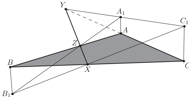
Figure 3.3B. The 3D proof of Menelaus's theorem.
