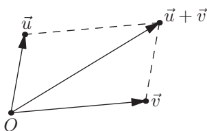
Figure A2. Adding two vectors.
