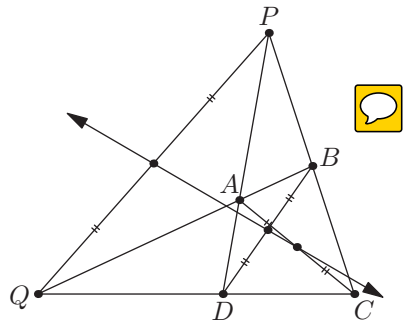
Figure 10.3A. The Gauss line.
