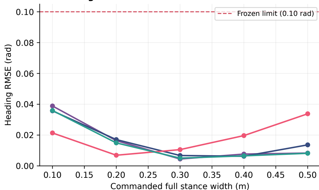
d Heading remains forward
