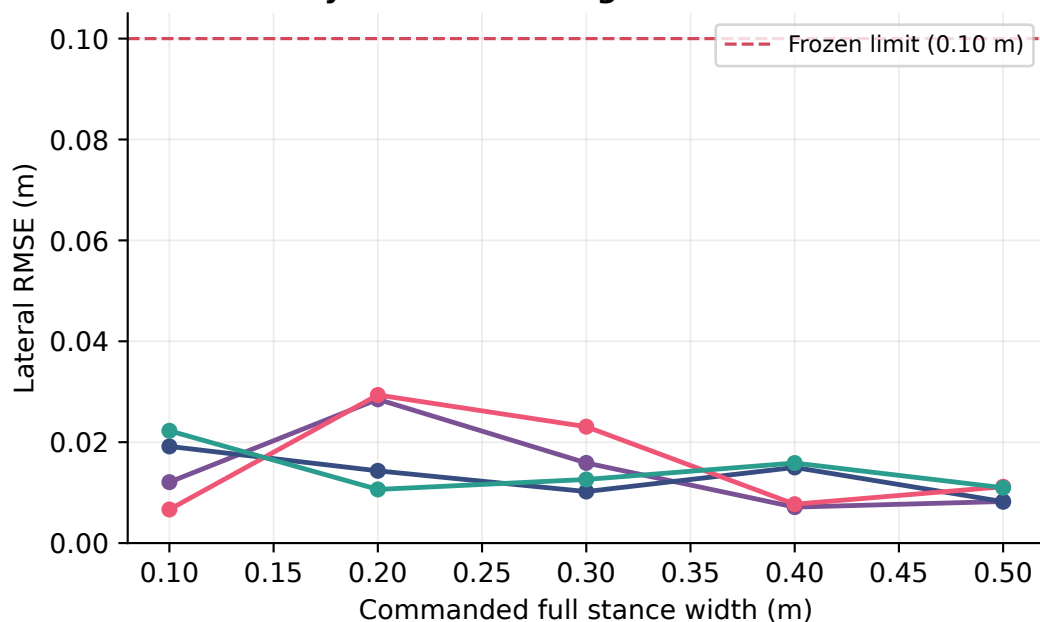
c Robot stays near the straight line
