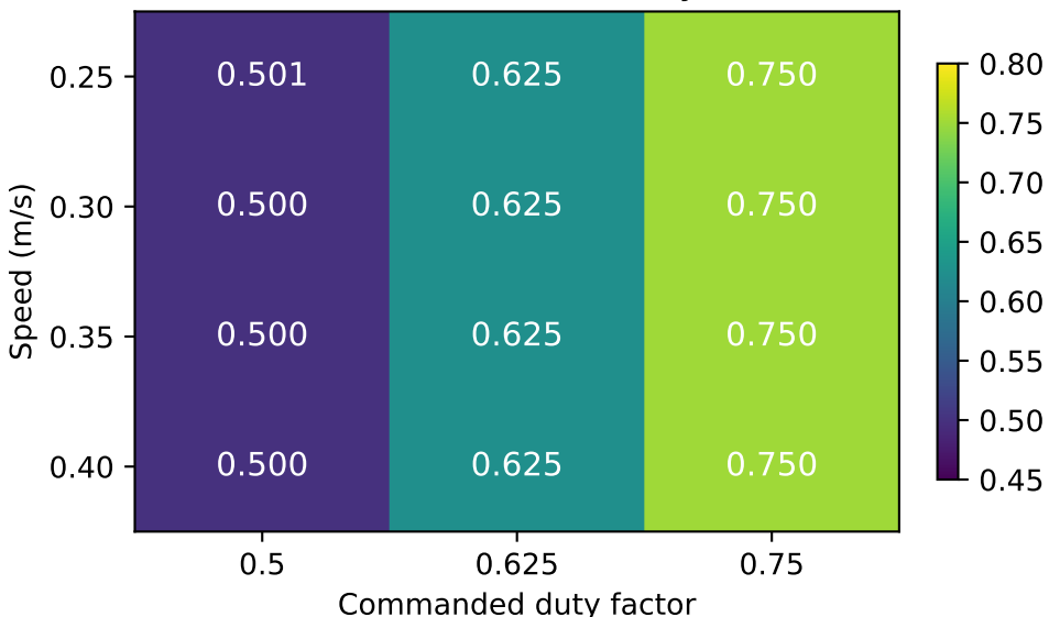
Trot — Command/contact/energy compliance
