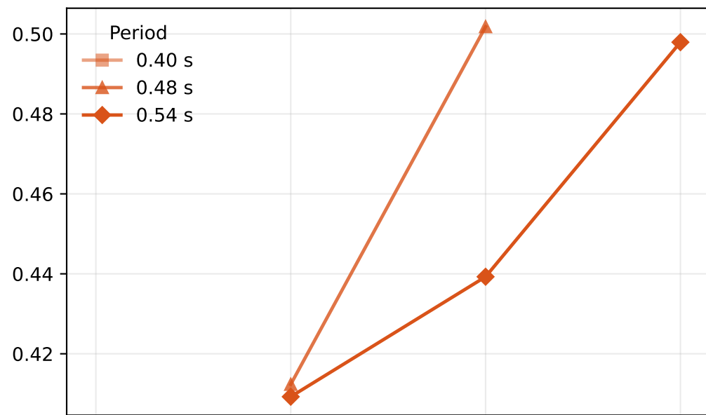
Walk
