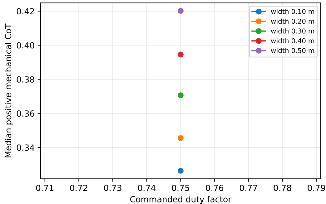
Walk, speed 0.35 m/s, period 0.48 s
