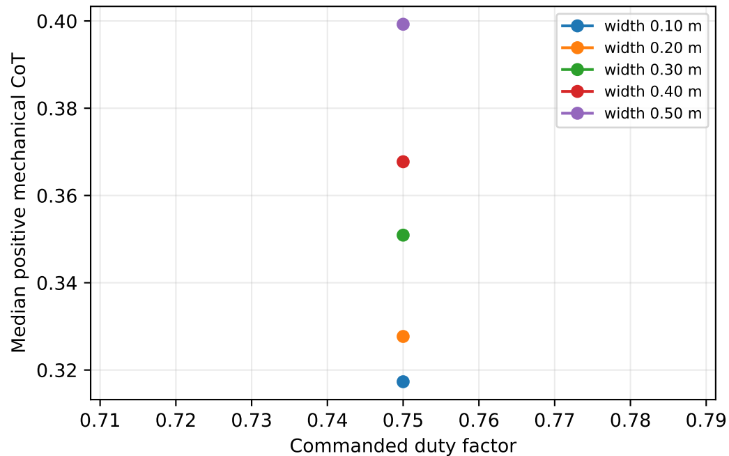
Walk, speed 0.40 m/s, period 0.48 s
