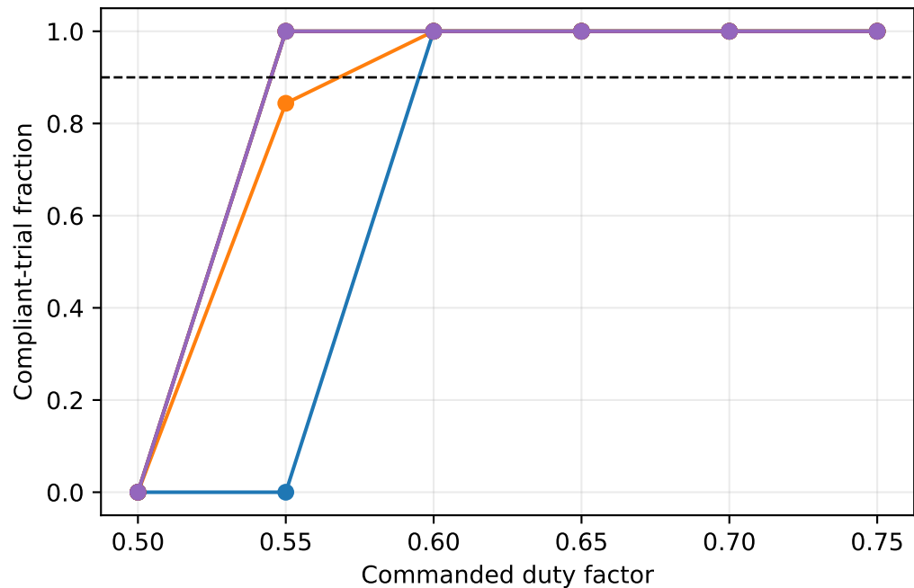
Trot, speed 0.35 m/s, period 0.48 s
