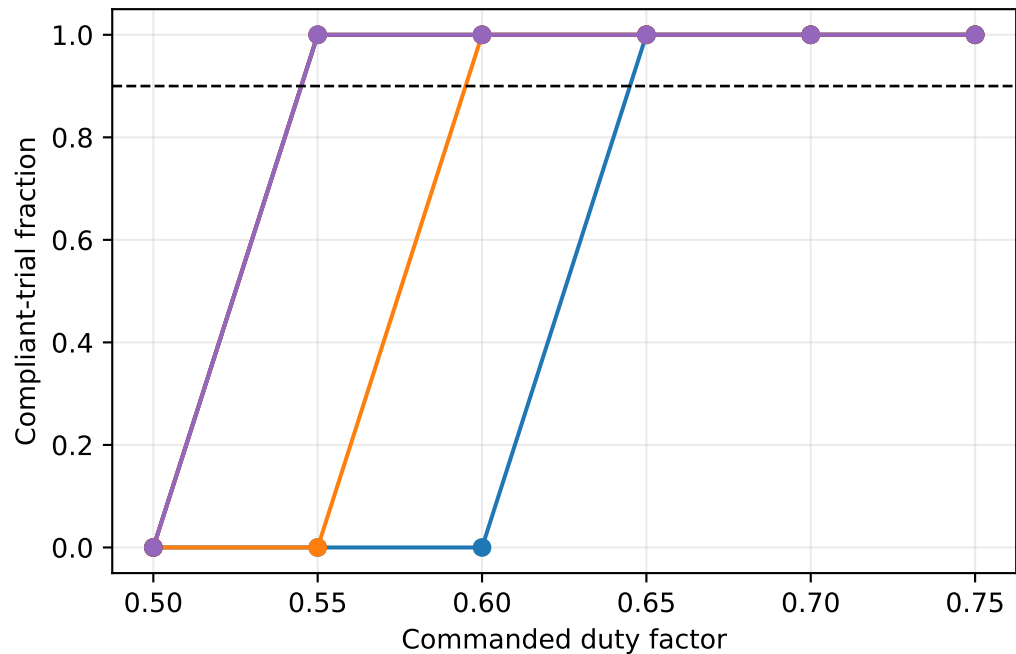
Trot, speed 0.25 m/s, period 0.48 s
