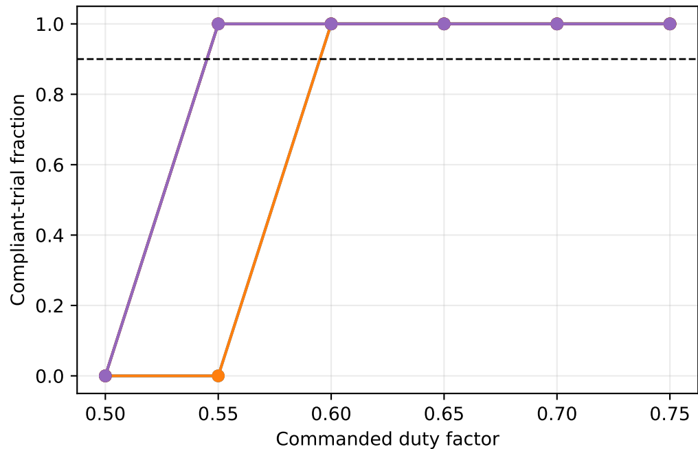
Trot, speed 0.30 m/s, period 0.48 s
