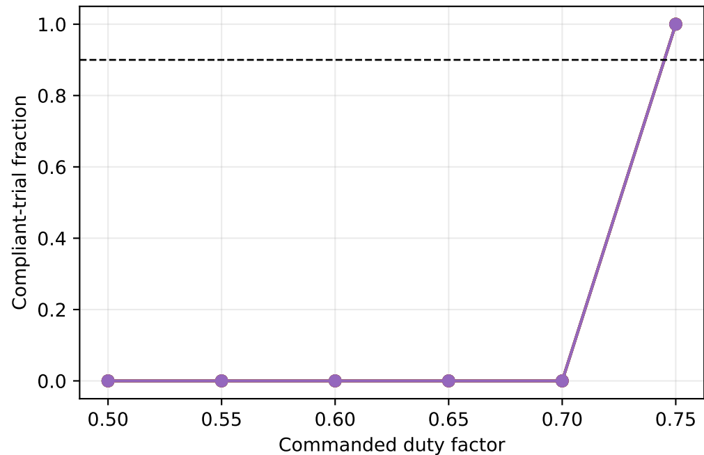
Walk, speed 0.35 m/s, period 0.48 s
