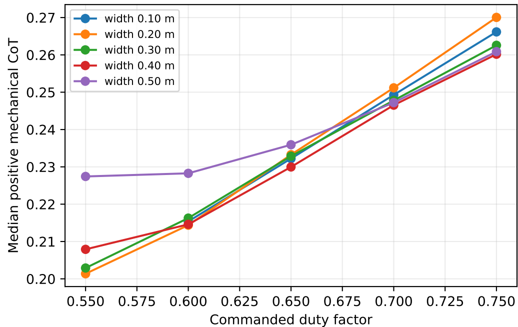
Trot, speed 0.35 m/s, period 0.48 s
