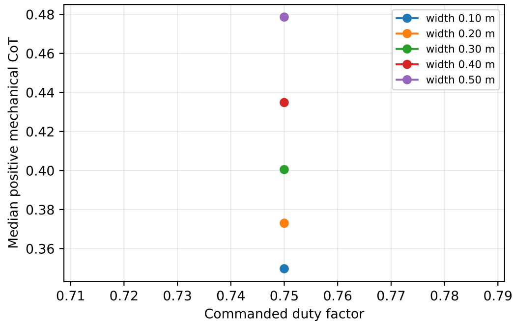
Walk, speed 0.30 m/s, period 0.48 s
