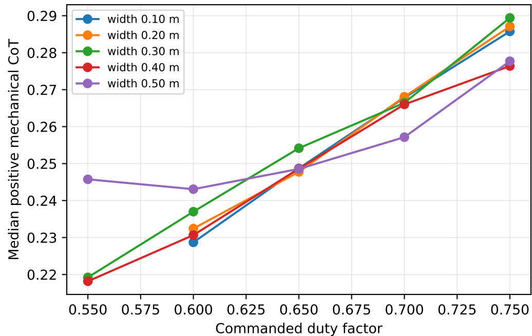
Trot, speed 0.30 m/s, period 0.48 s
