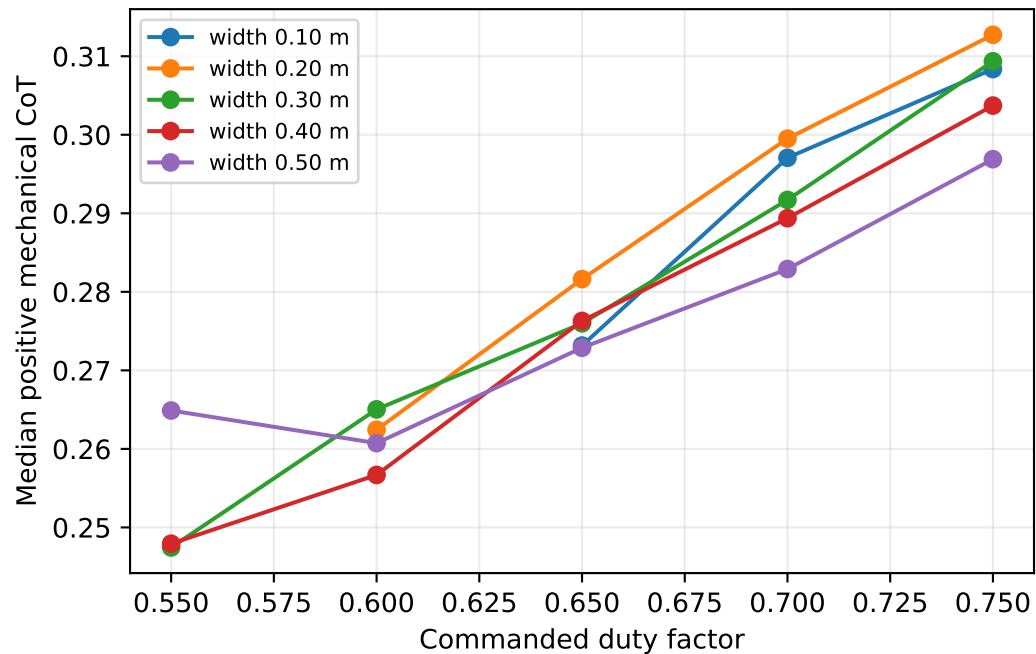
Trot, speed 0.25 m/s, period 0.48 s
