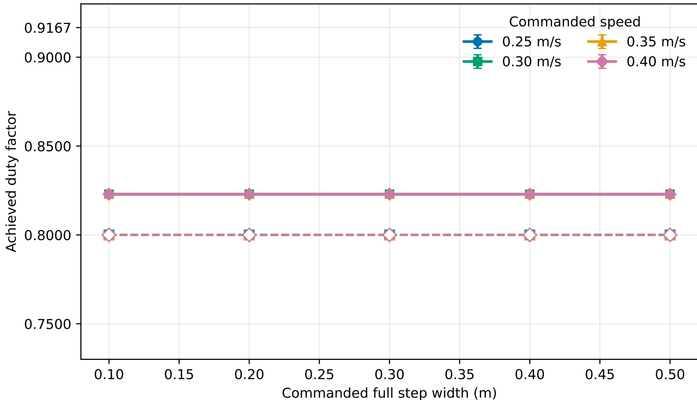
High-duty walk validation, period 0.48 s Dashed open markers: selected; solid filled markers: achieved
