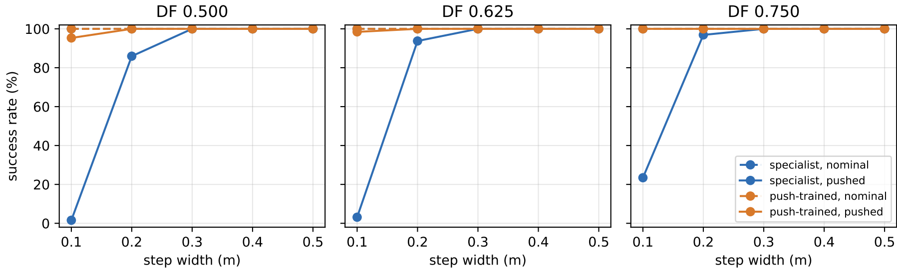
trot: success by step width, period 0.48 s, 0.30 m/s
