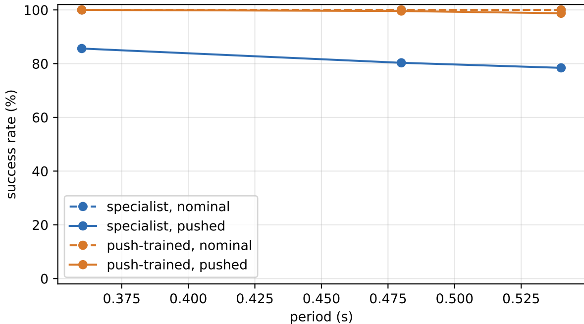
trot: success vs period (s) (speed 0.30)
