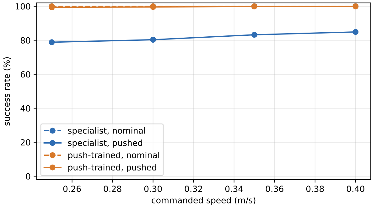
trot: success vs commanded speed (m/s) (period 0.48)
