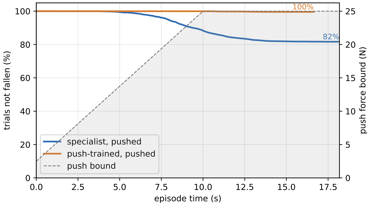
trot: survival under ramped push
