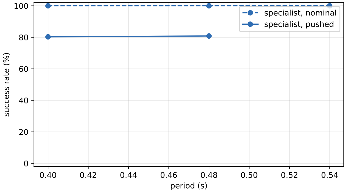
walk: success vs period (s) (speed 0.30)
