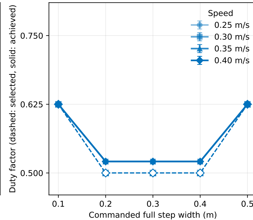
Walk, period 0.48 s
