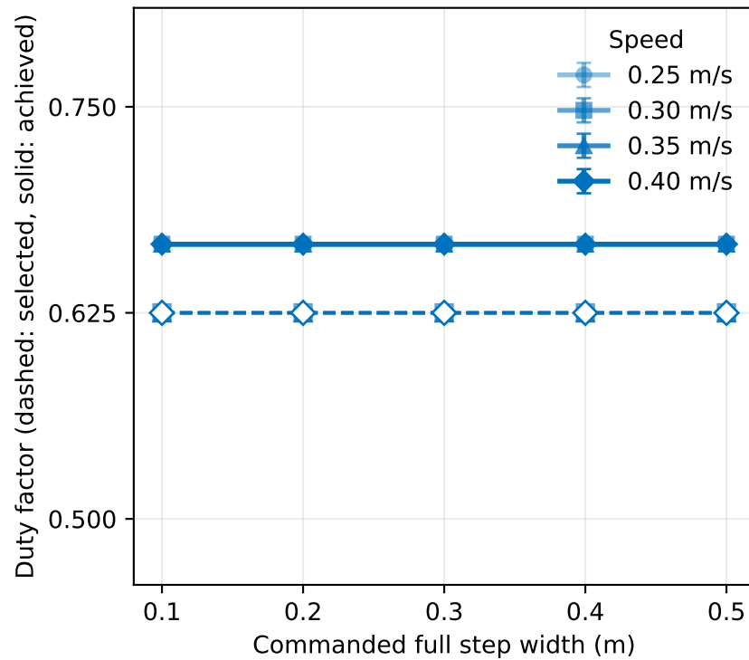
Trot, period 0.36 s
