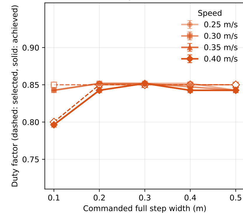
Walk, period 0.54 s
