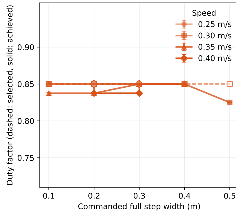
Walk, period 0.40 s
