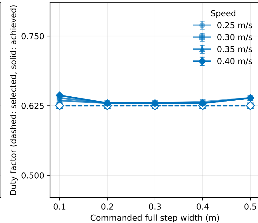
Walk, period 0.54 s
