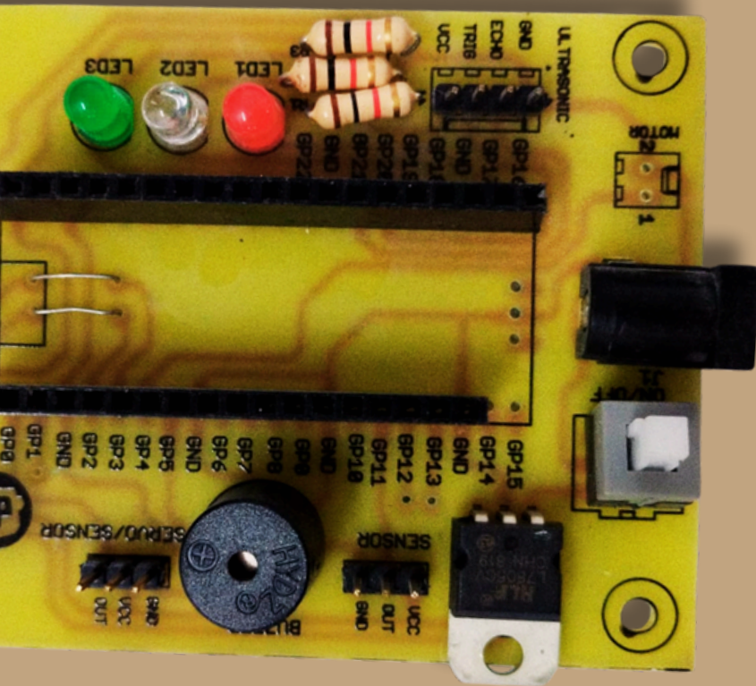
RPi Extn Board
