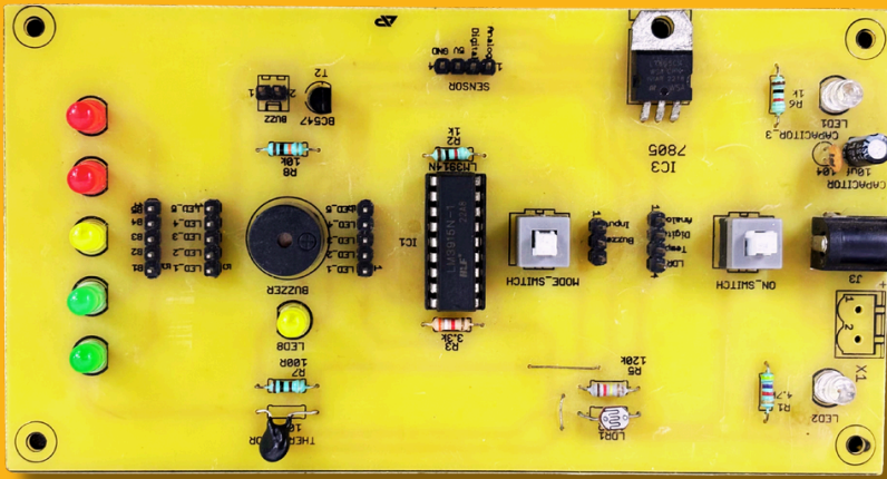
Masterboard
