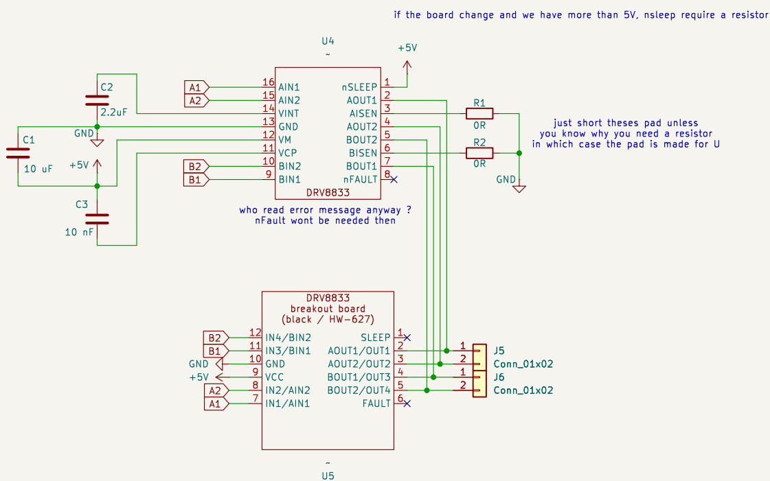
DC motor Driver
