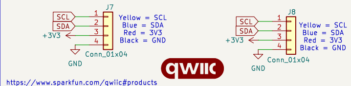
3V3 I2C connector (QWIIC)
