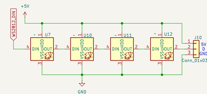
WS2812 RGB addressable LED
