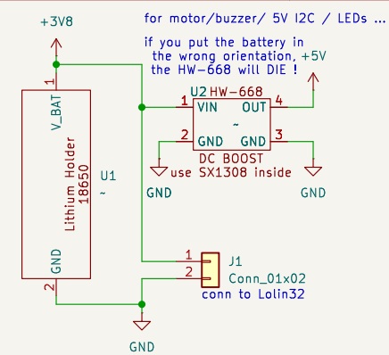
Lithium Cell + DC Boost
