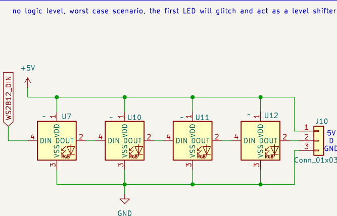
WS2812 RGB addressable LED
