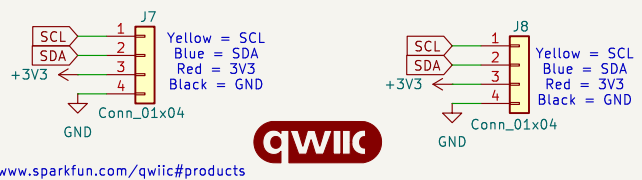
3V3 I2C connector (QWIIC)
