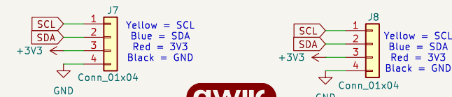
3V3 I2C connector (QWIIC)
