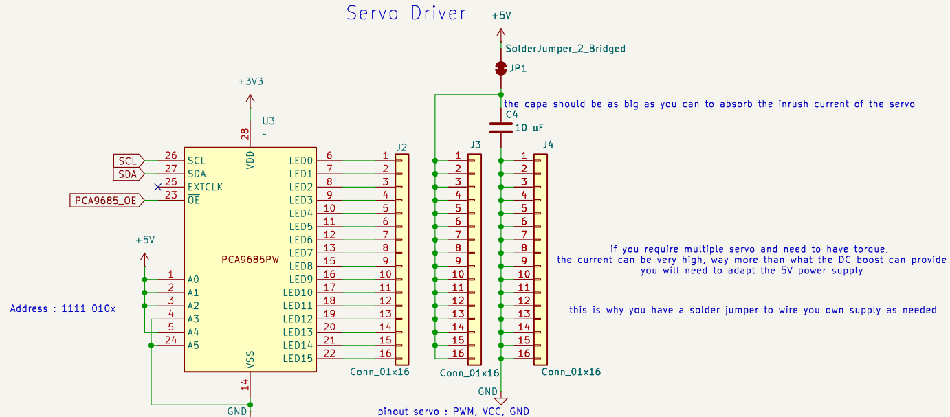
Servo Driver
