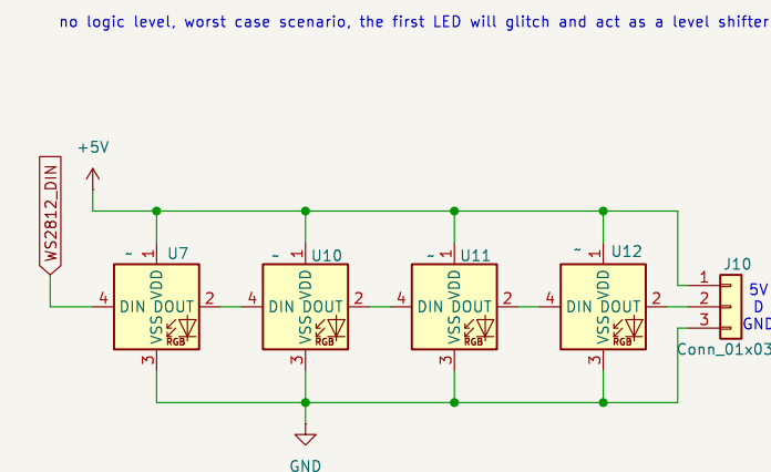
WS2812 RGB addressable LED
