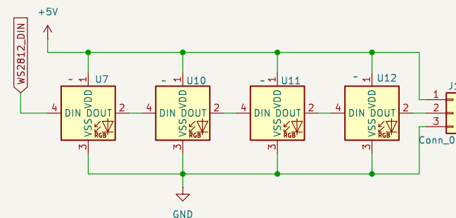
WS2812 RGB addressable LED
