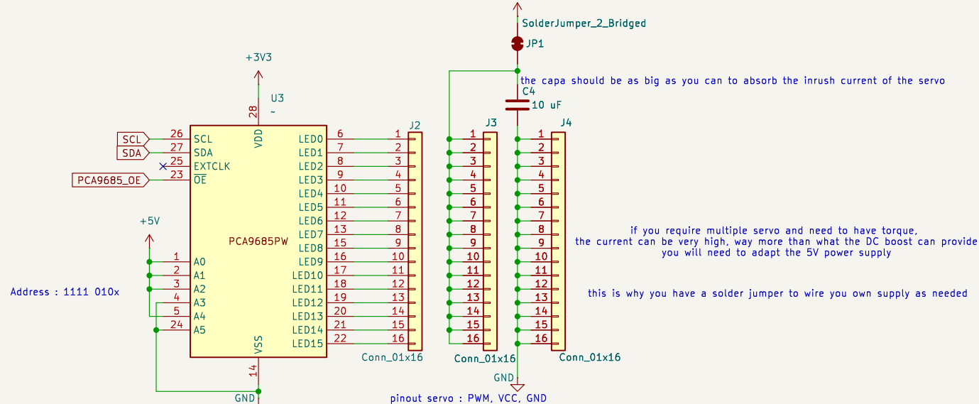
Servo Driver
