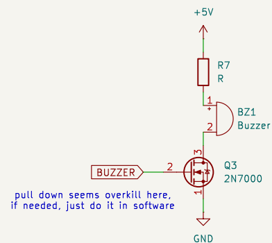
Buzzer
