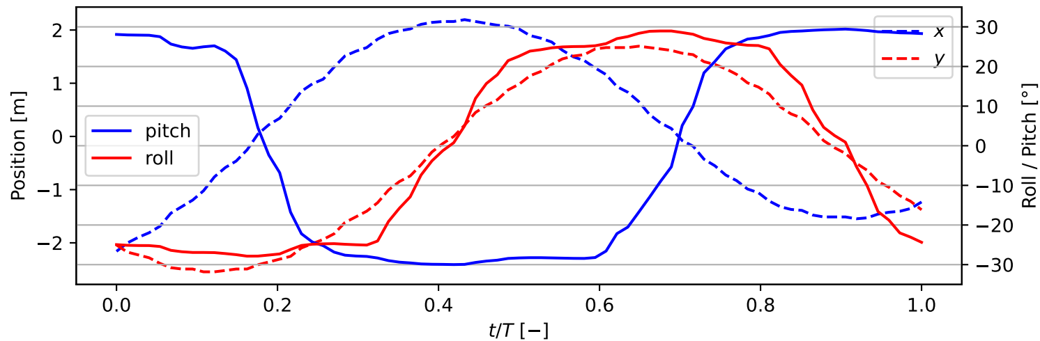
Circular Trajectory r = 3m , v = 5m/s
