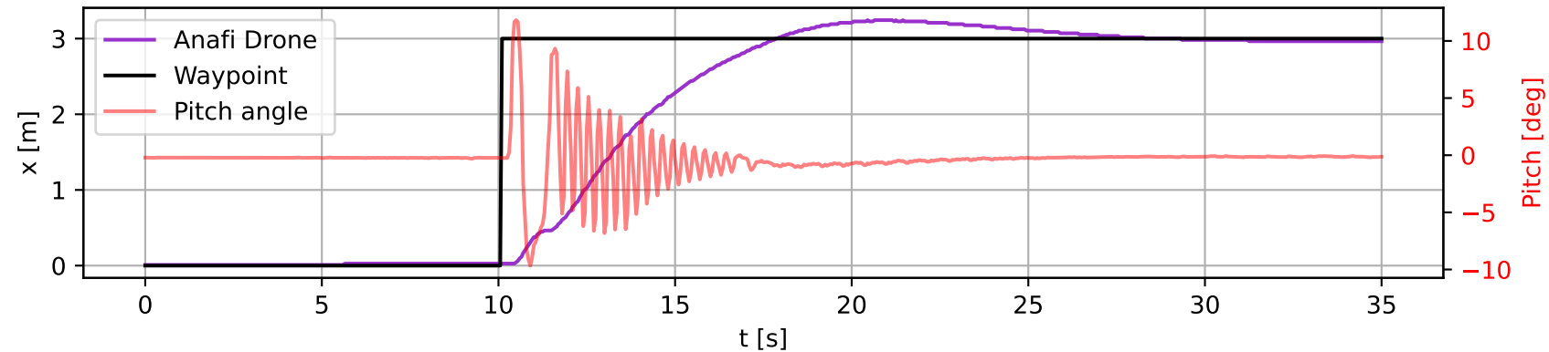
Waypoint Tracking (x-Direction)
