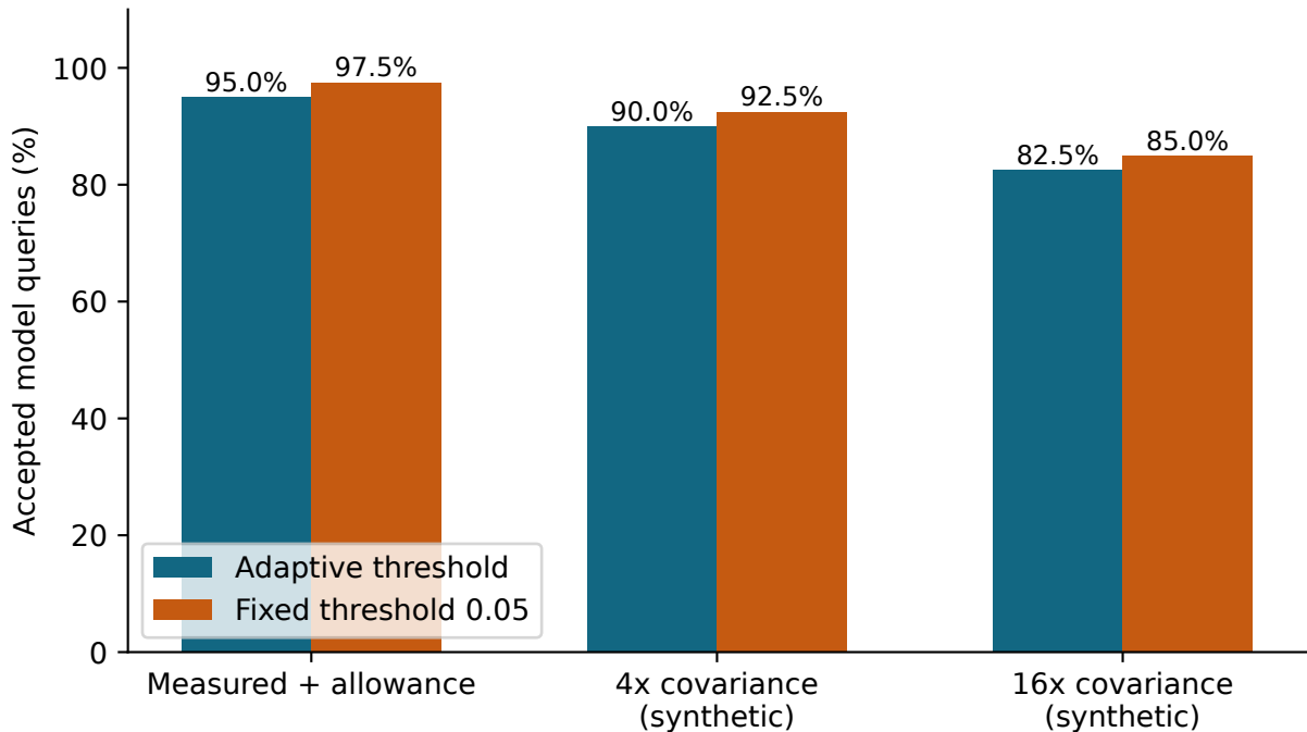
Matched policy comparison: 120 cases per regime
