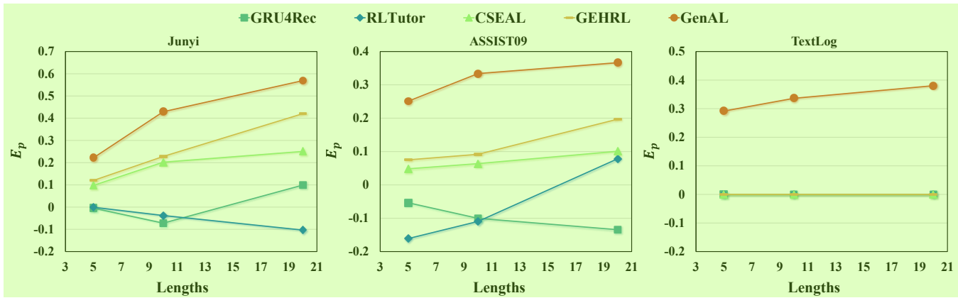
Figure 3: Impact of different lengths on three datasets with representative baseline models and our GenAL. It should be noted that the baseline models failed to achieve the learning goals in TextLog, so we present their results as 0.00.
