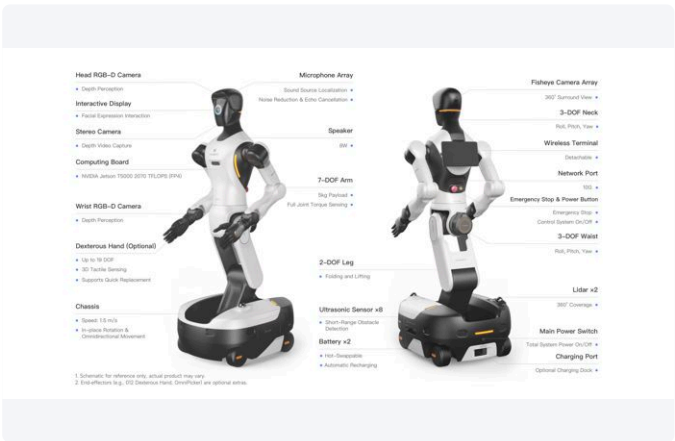
Genie G2 精灵G2 AgiBot (Zhiyuan Robotics) · China · shipping
