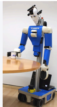
Cosero Cosero (Cognitive Service Robot); predecessor Dynamaid University of Bonn — NimbRo · Europe · discontinued
