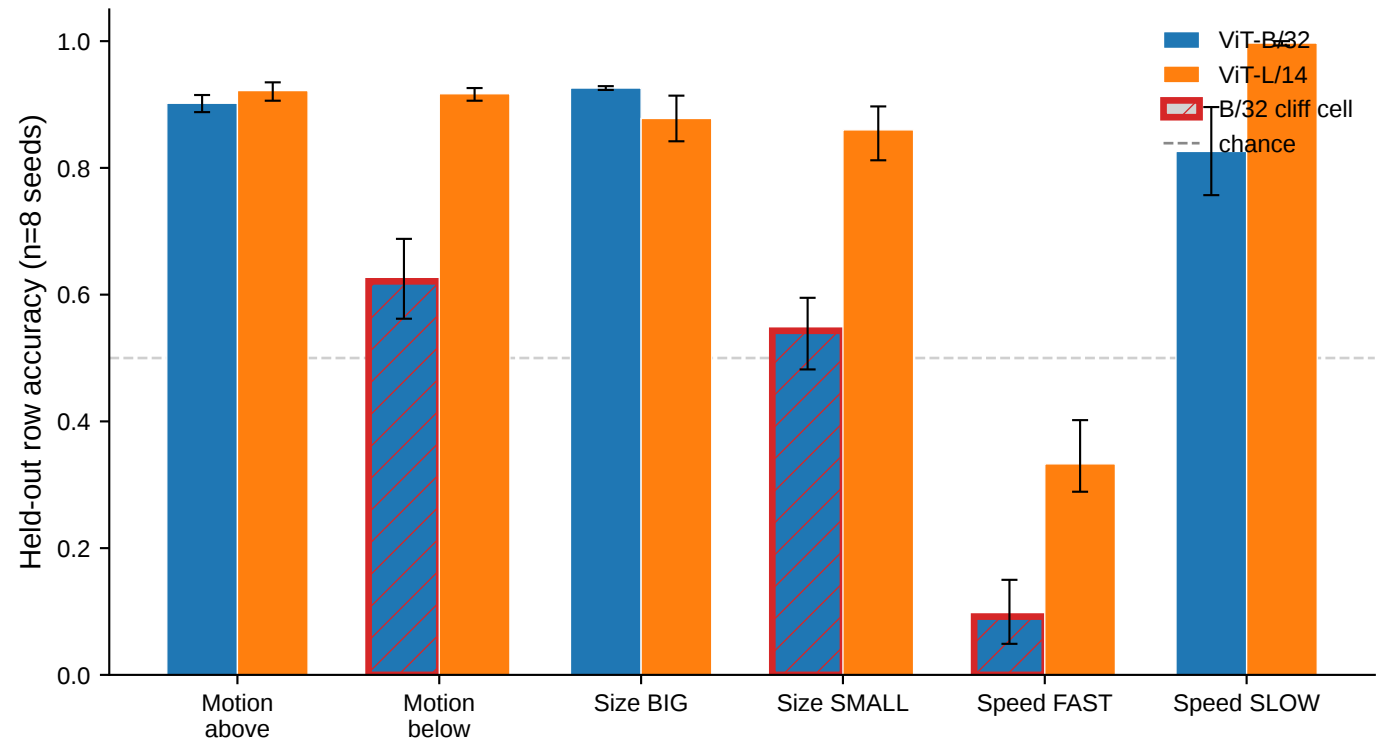
Three-axis \times two-architecture cliff matrix (n=8 seeds)
