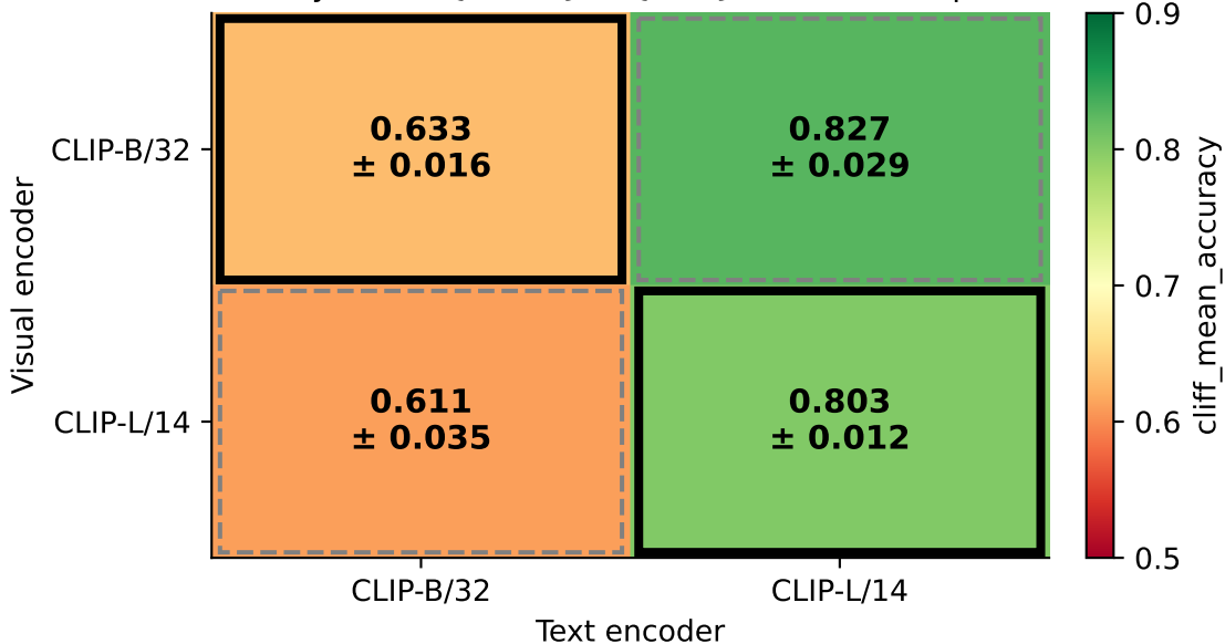
Cliff accuracy under {visual} × {text} encoder swaps (3 seeds)
