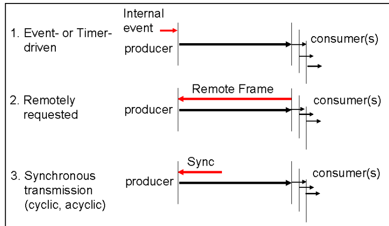
Fig 1.: PDO Transmission principles
