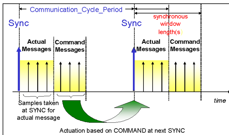
Fig 2.: CANopen Sync Mechanism
