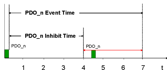
Fig 4: TxPDO Time Window
