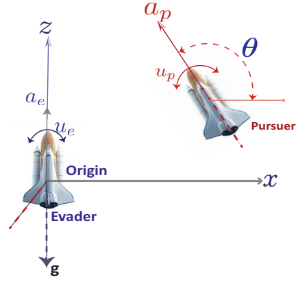
Fig. 1. Motion of two rockets on a Cartesian \mathbf{xz} -plane with a thrust inclination in relative coordinates given by \theta := u_p - u_e .
