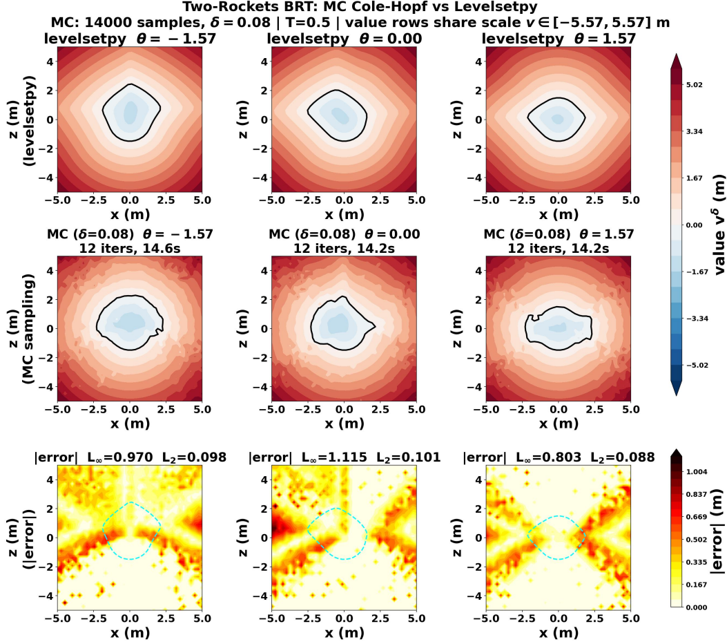
Figure 1: 2D BRT slices for specific relative heading angles \theta = \{-90^\circ, 0, 90^\circ\} of two rockets on a plane as derived in [Molu, 2024b]. The top row depicts the classical grid-based resolved levelsets using the classical grid-based solver in [Molu, 2024b] vs our Monte Carlo solver (middle row). The top two rows plot the value function v^\delta (m) on a single shared, zero-centered diverging color scale (common colorbar at right) so the two solvers are directly comparable; the blue-cyan-red contours signify up to 20 levelsets of divergence from the zero levelset (black contours), the field being negative inside the capture region (radius 1.5) and positive outside. The bottom row is a heat map of the pointwise errors at each relative orientation \theta (its own colorbar). Notice that errors are largest near the boundary of the usable part where the absolute gradient of the value function |Dv^\delta| is largest. This figure shows a single representative Monte Carlo seed for visual clarity.
