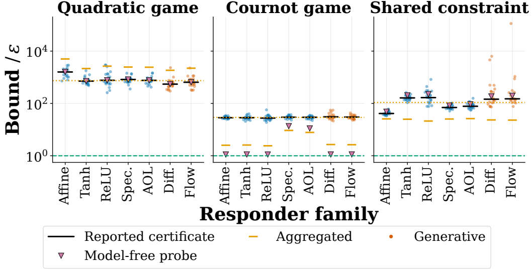
Fig. 4: Tightness by response family. Certified bound over true exploitability, dots seeds and bars medians, log scale; panels are the quadratic, Cournot and shared-constraint games. Blue marks families with a rigorous Lipschitz bound, orange those without.
