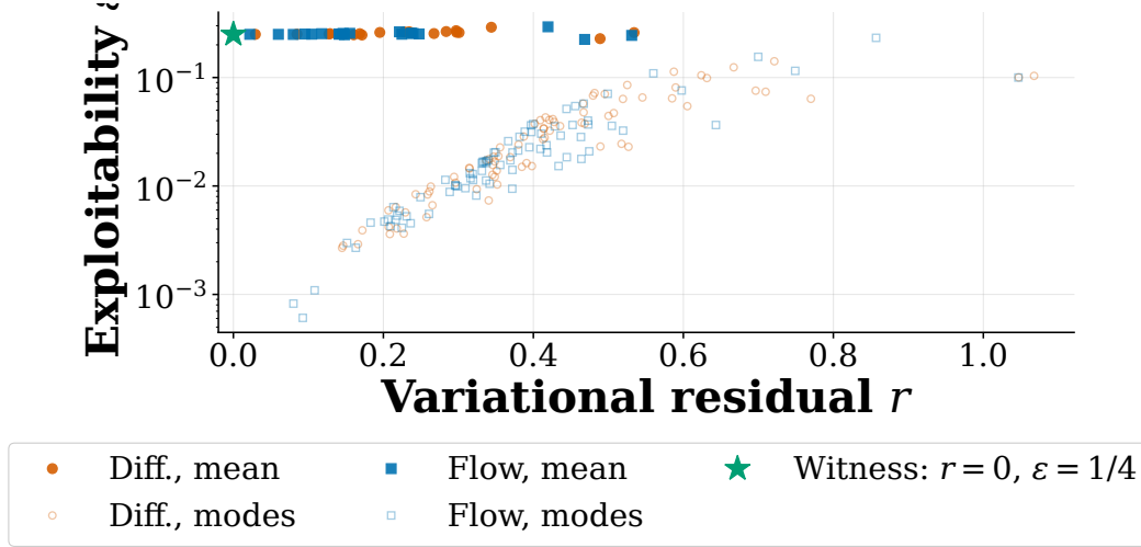
Fig. 7: A vanishing residual is no evidence of a small gap. Exploitability against variational residual on the bimodal witness of Proposition 3.2, log ordinate, 20 seeds per family. Filled markers are the conditional-mean fixed points, hollow markers the four mode-selected profiles per seed, and the star is the analytic witness, at residual exactly zero and exploitability 1/4 . Mode selection moves the cloud down and to the right of the conditional-mean profiles it improves on, so that a smaller gap is bought at a larger residual. Within the mode-selected cloud the two quantities are positively associated; it is the shift between the groups that the plane shows.
