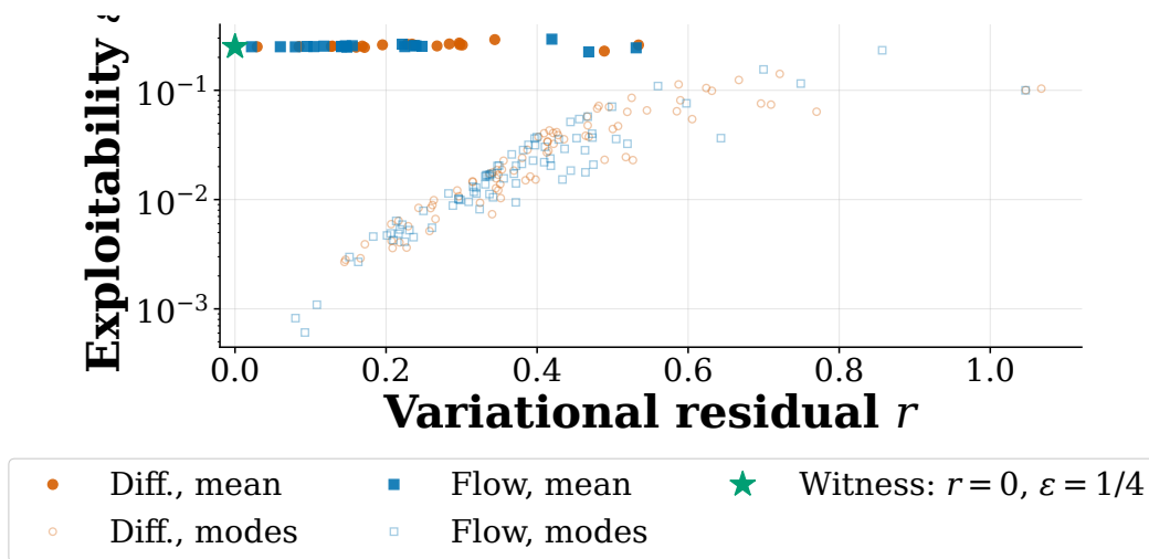
Fig. 7: A vanishing residual is no evidence of a small gap. Exploitability against variational residual on the bimodal witness of Proposition 3.2, log ordinate, 20 seeds per family. Filled markers are the conditional-mean fixed points, hollow markers the four mode-selected profiles per seed, and the star is the analytic witness, at residual exactly zero and exploitability 1/4 . Mode selection moves the cloud down and to the right of the conditional-mean profiles it improves on, so that a smaller gap is bought at a larger residual. Within the mode-selected cloud the two quantities are positively associated; it is the shift between the groups that the plane shows.
