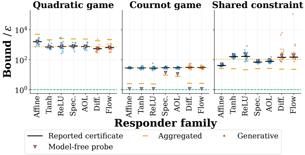
Fig. 4: Tightness by response family. Certified bound over true exploitability, dots seeds and bars medians, log scale; panels are the quadratic, Cournot and shared-constraint games. Blue marks families with a rigorous Lipschitz bound, orange those without.
