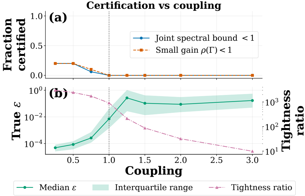
Fig. 5: Coupling sweep across the monotone boundary. Coupled quadratic game; the coupling parameter sets \lambda_{\min} of the symmetrized pseudo-gradient Jacobian exactly, so the grid crosses monotonicity at one.
