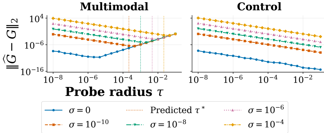
Fig. 6: Probe error against probe radius. Central-difference error in estimating \Phi_i versus \tau , at several noise scales \sigma ; medians over twelve probe points and twenty-four noise replicates each.
