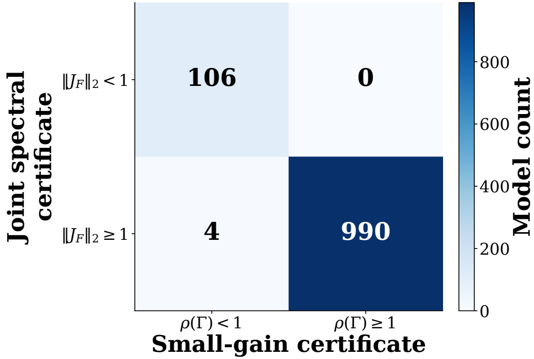
Fig. 8: Joint-spectral against small-gain certification on trained models. Contingency counts pooled over games and seeds, over 1100 certifiable trained models: 106 certified by both, 4 by small gain alone, 0 by the joint bound alone, and 990 by neither. The empty cell is a fact about these fits and not a dominance relation: \rho(\Gamma) \leq \|J_F\|_2 held in all 1100 of them, with a median gap of 0.040, so the skew-coupling direction that separates the two conditions analytically does not arise here at any threshold. This licenses no claim that either certificate dominates.
