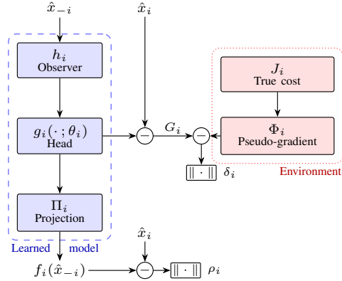
Fig. 1: A learned response map, and the game it is fitted to. Both G_i (6) and \rho_i (9) are differences from the same \hat{x}_i ; \delta_i is the consistency error, the one discrepancy that cannot be formed from the model alone.
