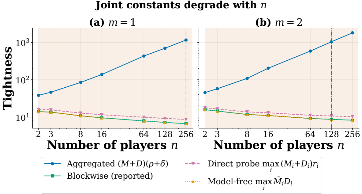
Fig. 2: Joint constants degrade with the player count; playerwise ones do not. Coupled quadratic game, (a) scalar and (b) two-dimensional actions, medians over 20 seeds, log–log, lower is tighter.
