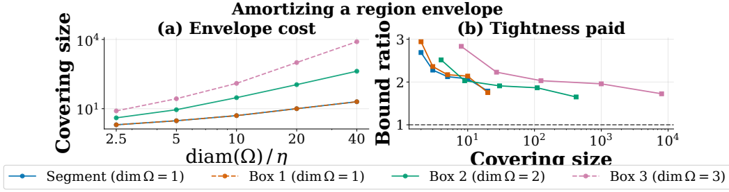
Fig. 3: Regional envelope costs and tightness. Medians over 10 seeds and 256 held-out profiles per region. (a) Covering size=break-even certified profile numbers. (b) Amortized bound over pointwise bound; the dashed rule is the value a single-profile probe attains.
