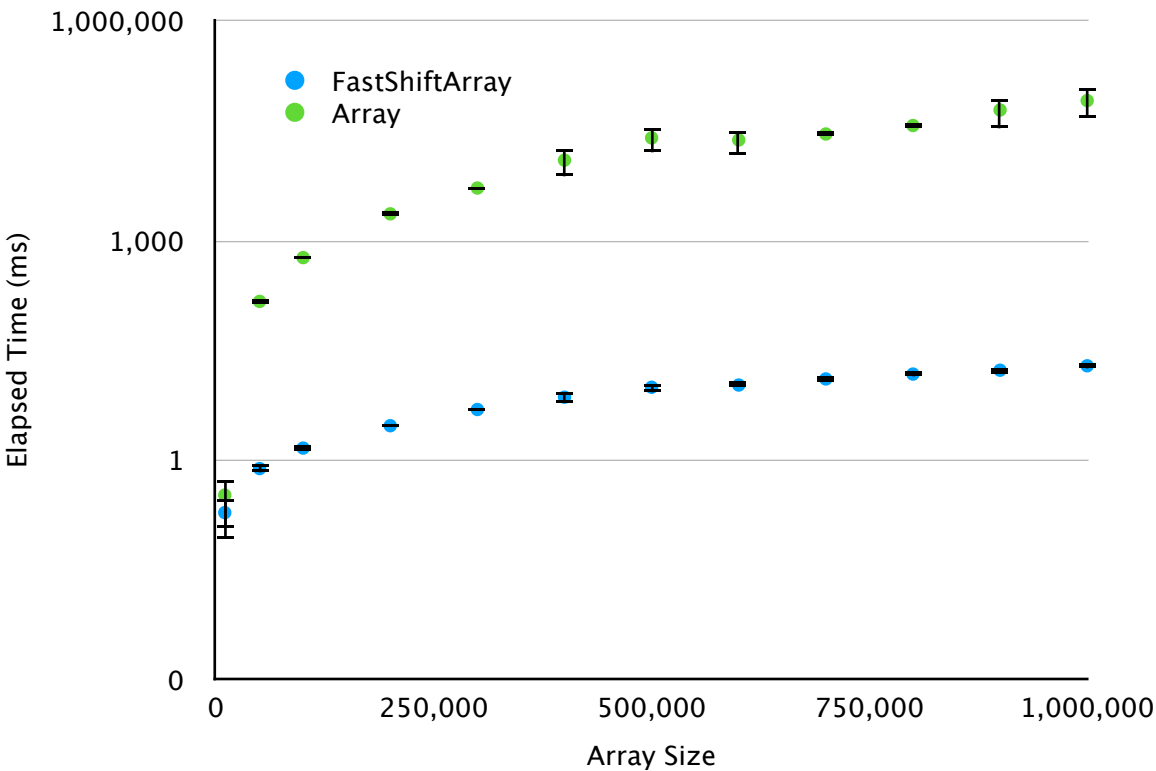
Performance of shift() (compacting = 100k)
