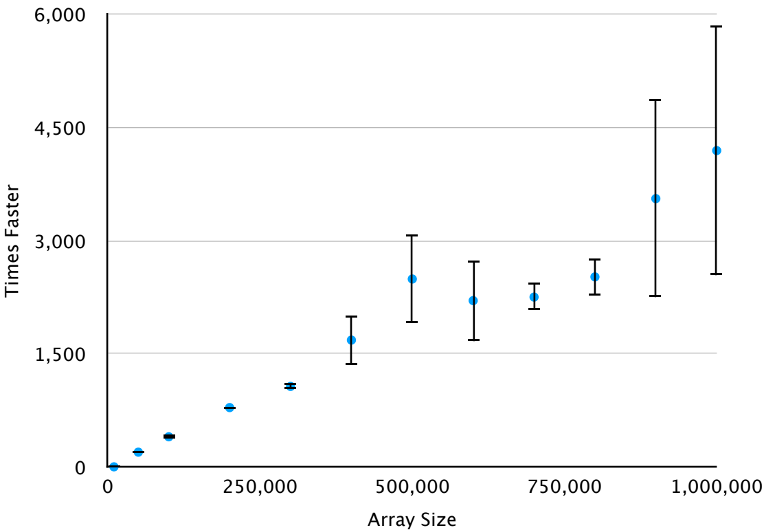
FastShiftArray shift() speed-up (compacting = 100k)
