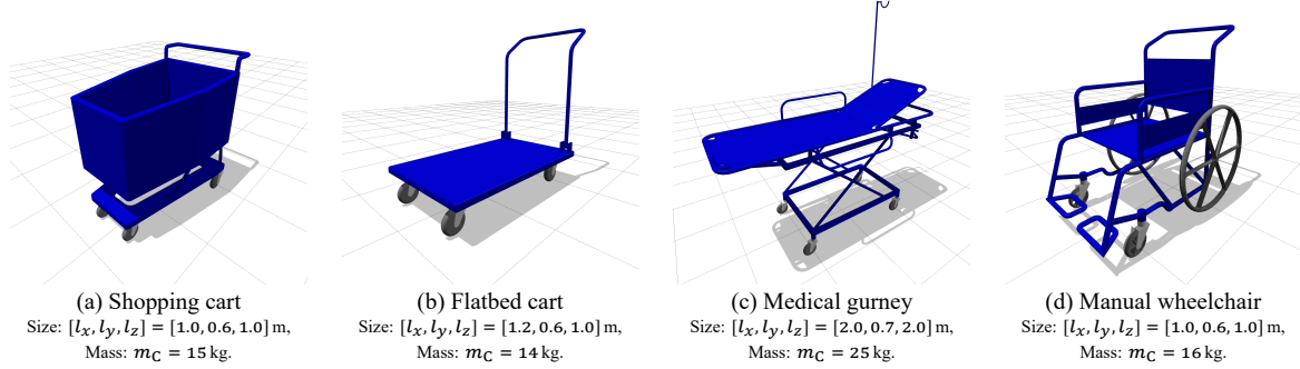
Fig. 3. Wheeled platforms evaluated in IsaacLab simulation.
