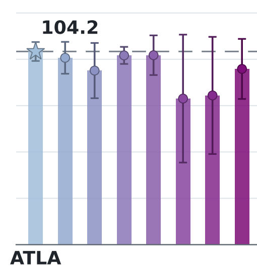
Credit latency
