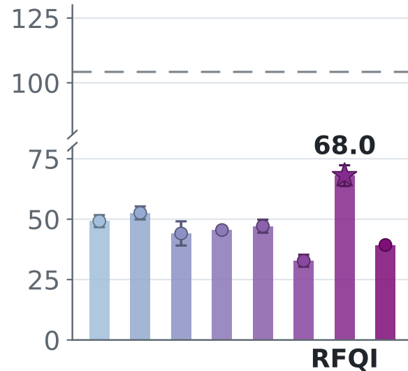
Observation
