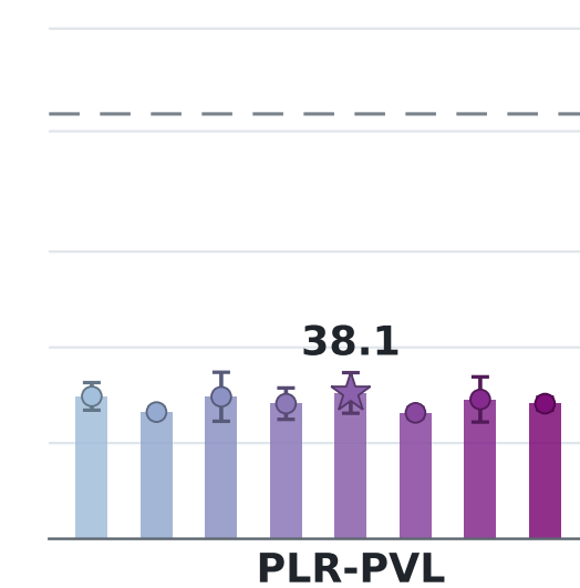
Action
