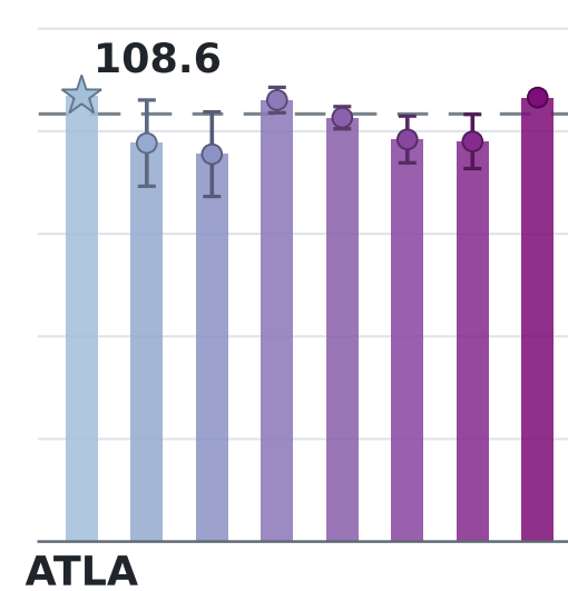
Reward
