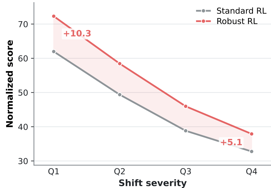
Robustness Decay
