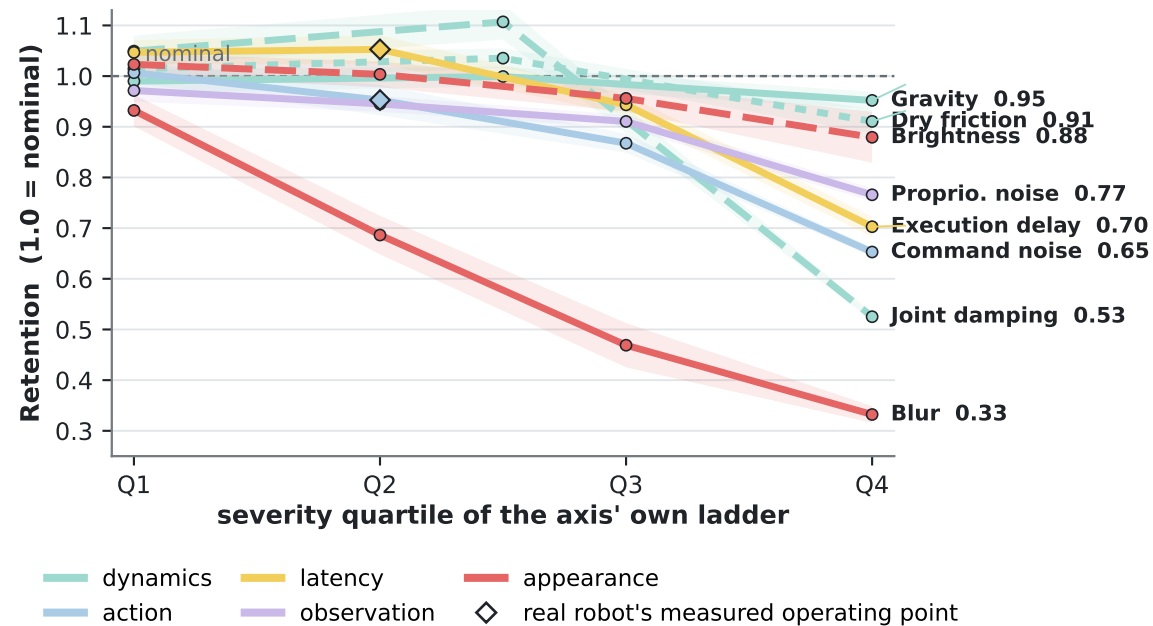
Performance degradation under shifts
