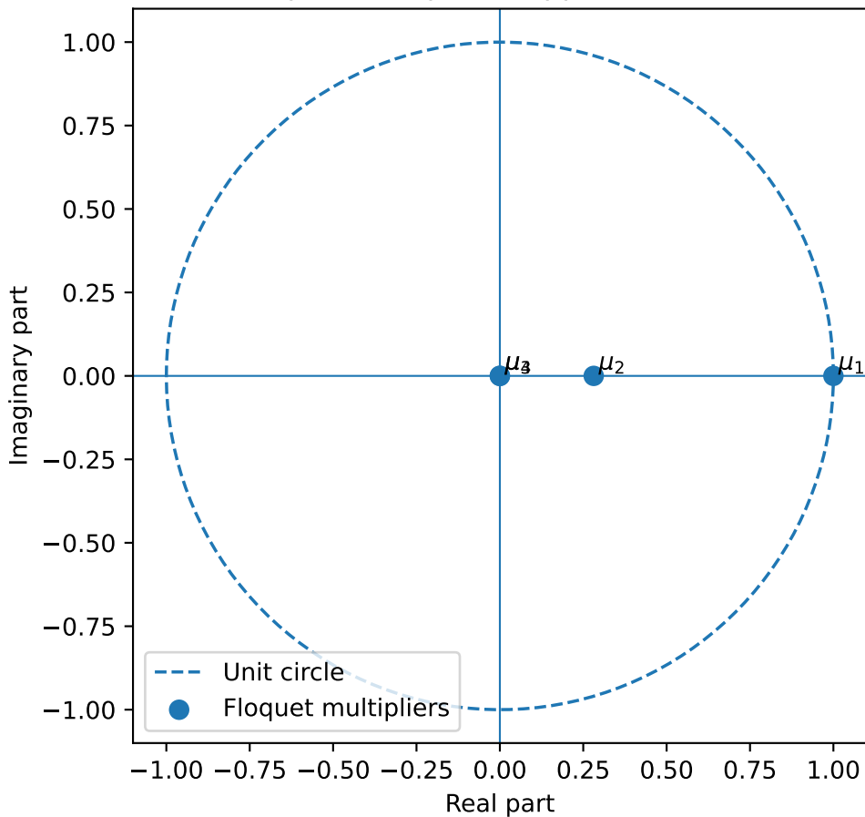
Floquet multipliers: applied scenario
