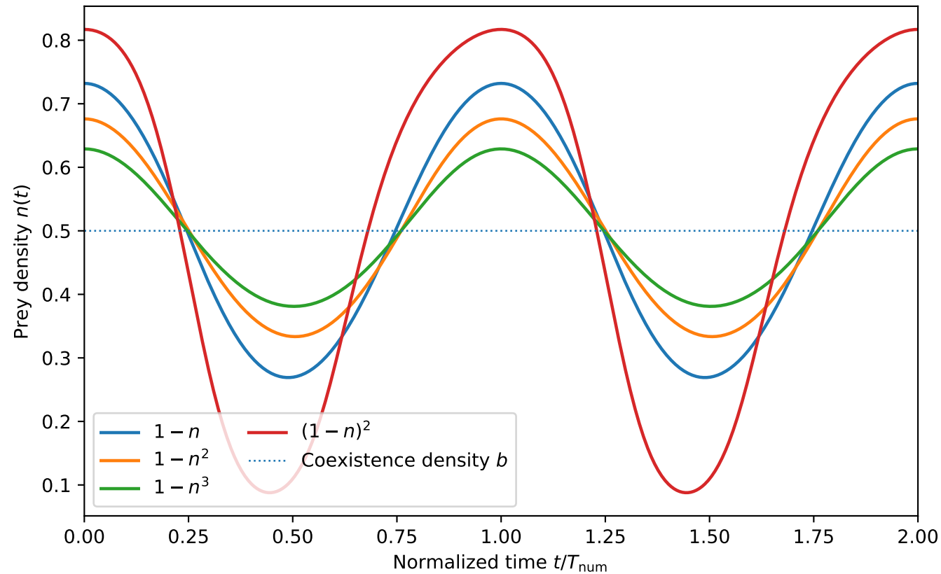
Stable prey oscillations at a = 0.94a_H
