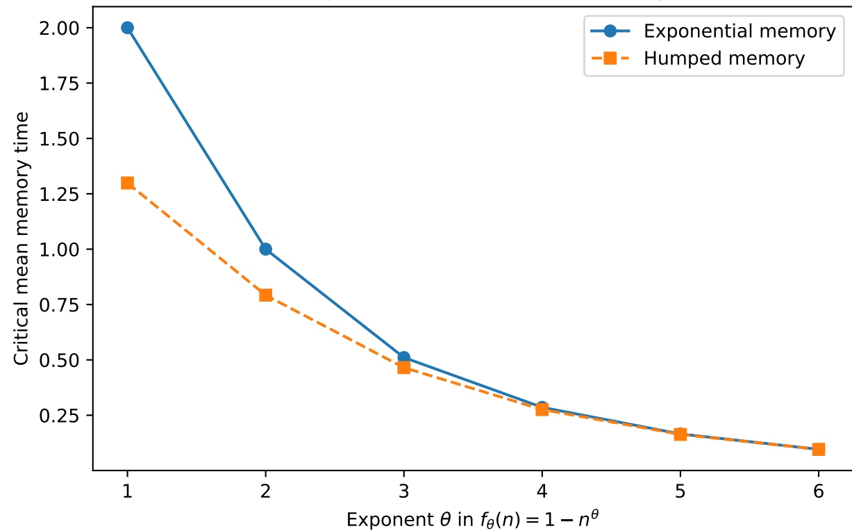
Kernel-dependent critical mean memory time
