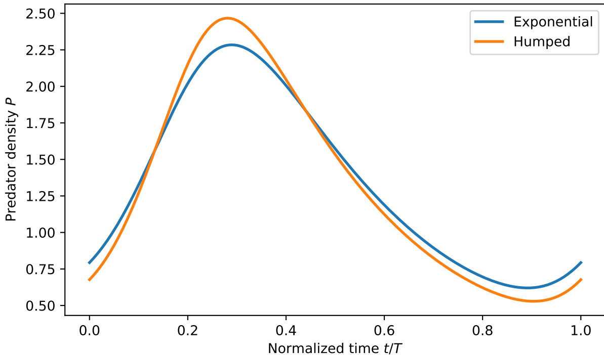
Predator density P over one periodic cycle
